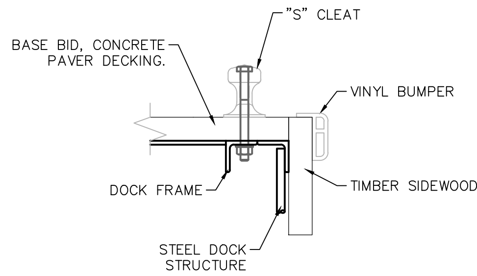
FENDER-CLEAT DETAIL
