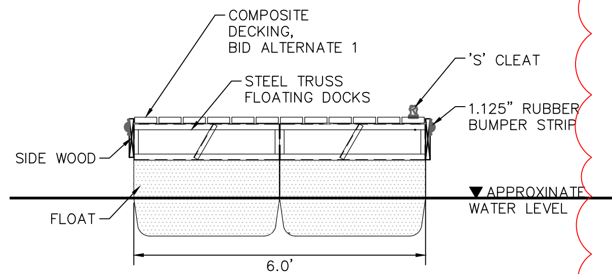
FLOATING DOCK SECTION
